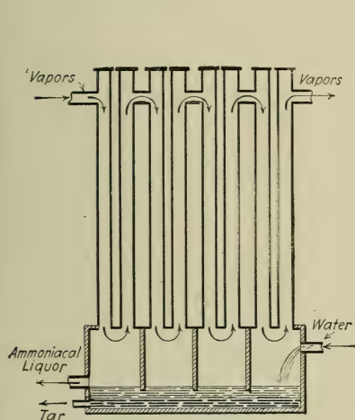
Fig. 59.—Air Condenser.
